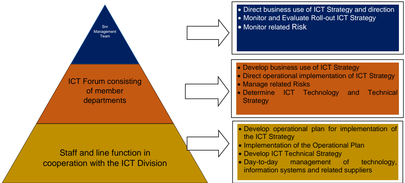
Diagram 1. CGICT Model
